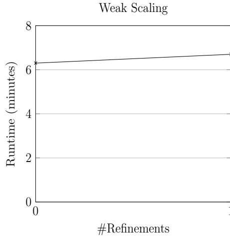
Figure 4: Weak Scaling for Spine-Dendrite simulation runs without ER (using our prior allocation COMET) present with respect to Refinement level and runtime. For 0 refinement, 24 procs. were used and for 1 refinement 192 procs. were used.
